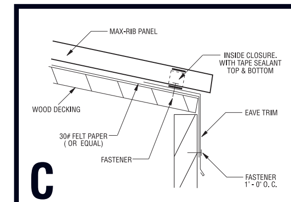
EAVE WITHOUT GUTTER
