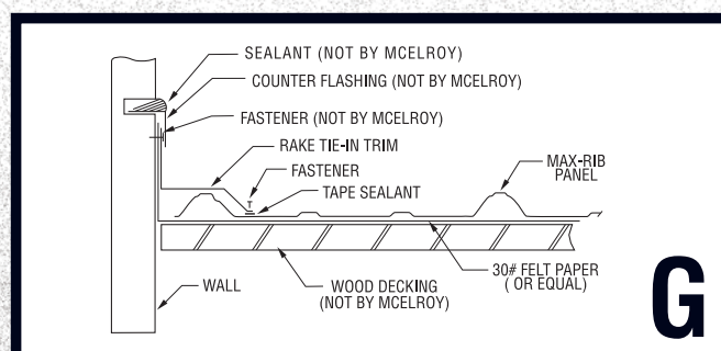
RAKE TIE-IN CONDITION
