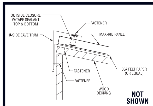
HIGH-SIDE EAVE CONDITION
