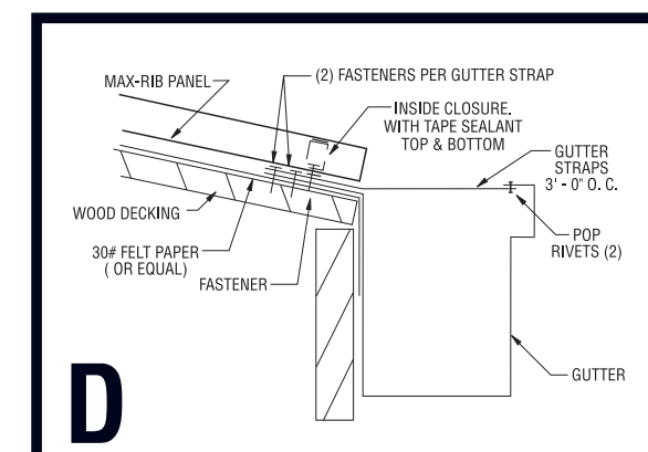
EAVE WITH STANDARD GUTTER
