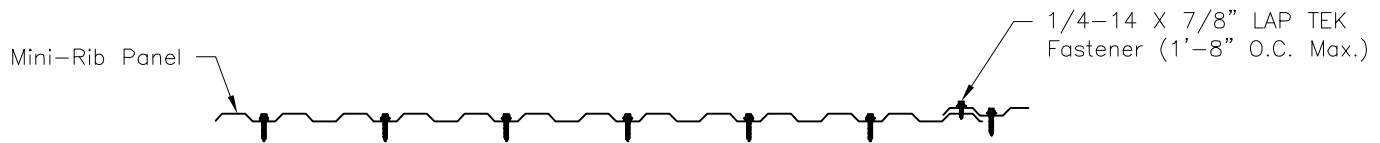
FASTENER PATTERN (@ Eaves, Ridges & Endlaps)
