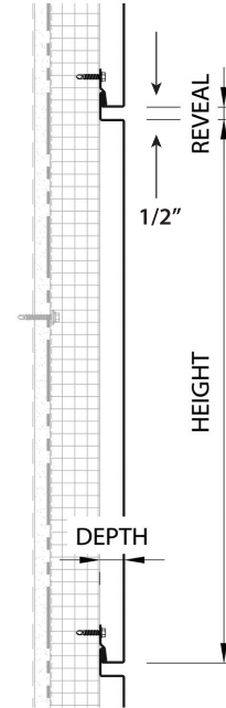
Visionline-F Series Vertical Detail
