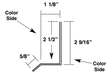
Fascia Base Trim VTFBT
