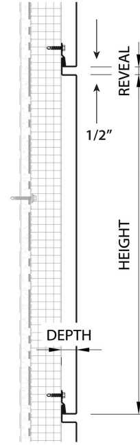
Visionline F Series Vertical Detail
