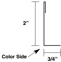
Cover Trim VTCT
