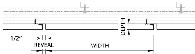
Visionline F Series Horizontal Detail
