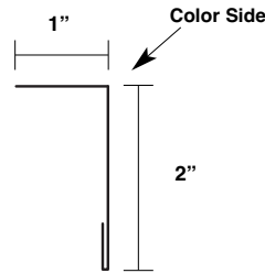
Inside Corner Trim VTIC
