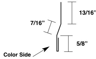
Panel Cleat VTPC
