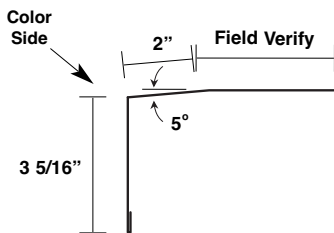
Sill Trim VTST
