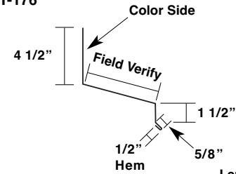
Wainscoat Flashing MT-176
