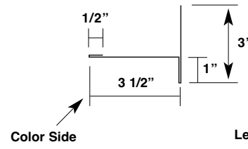
FW Zee Closure MT-178
