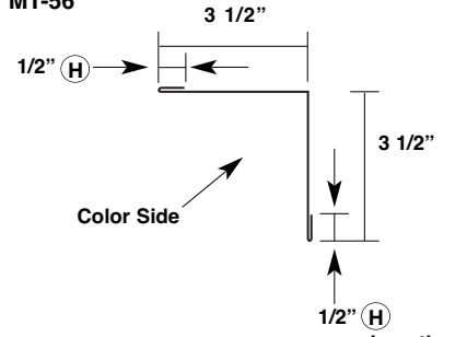
Inside Corner MT-56
