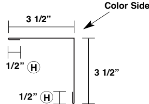
Outside Corner MT-55
