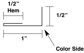
1 1/2" Sill Trim with Return MT-148
