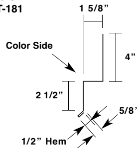
Zee Sill Trim MT-181
