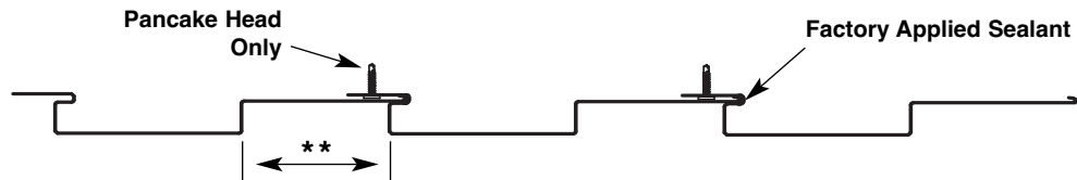
Custom Reveal Seam Engagement Pancake Head Fastener (Fastener Type as Required)
