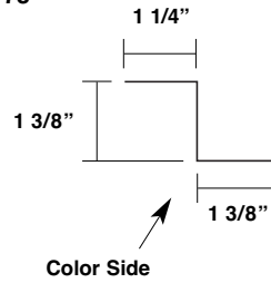
FW Zee Closure MT-178
