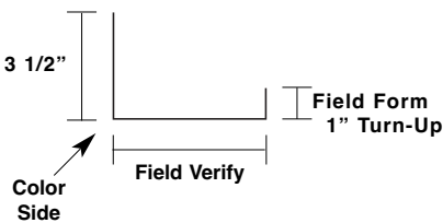
Head Trim MT-180
