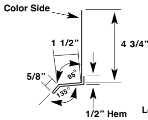
Sill Trim MT-177
