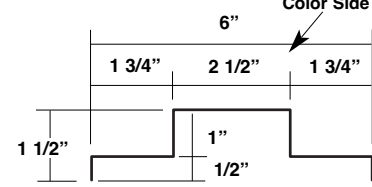
Counter Flashing Trim Item #: 38382
