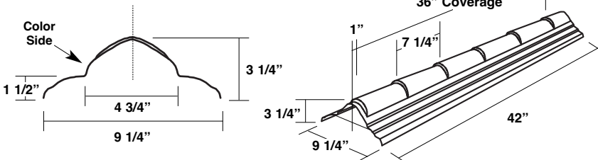
Contoured Ridge / Hip Trim Item #: 38395
