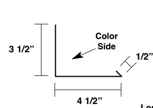
Cricket / Saddle Leg Item #: 38412
