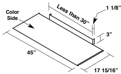
Commercial Gambrel Trim* Item #: 38431
