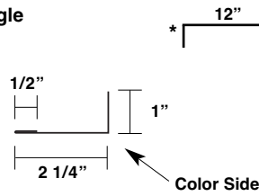
Outside Angle MQOA2
