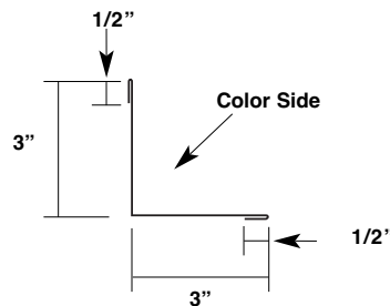
Inside Angle for Inside Corner 3" x 3" MQIA3
