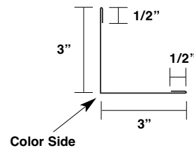
Outside Angle For Outside Corner 3" x 3" MQOA3
