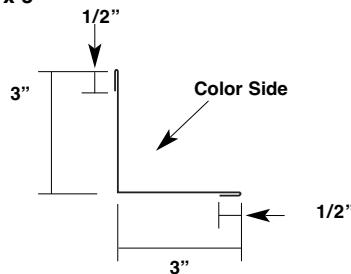
Inside Angle for Inside Corner 3" x 3"
