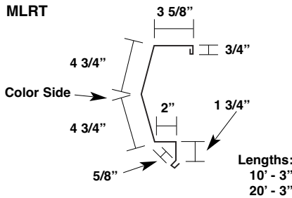
Rake Tie-In Trim
