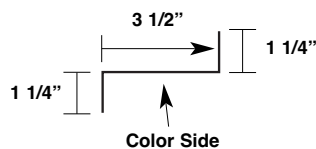
Insulation Zee Trim MLIZ
