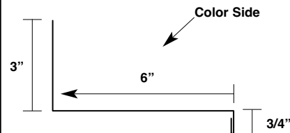
Alternate Rake Tie-In Trim
