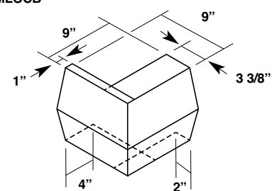
Outside Corner Box for Standard Gutter (Up to 2:12 Pitch) (Right Hand Shown - Left Hand Opposite) MLOCB
