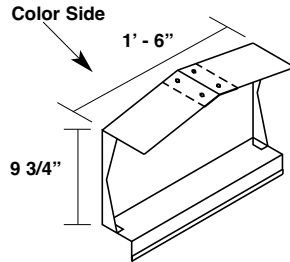
Fixed Peak Box (2:12 to 4:12 Pitch) MLFXPB4
