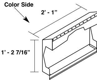
Floating Peak Box (Up to 2:12 Pitch) MLFLPB2
