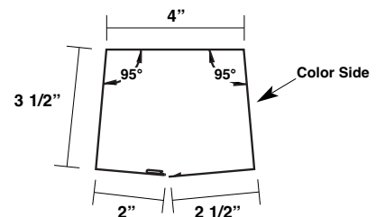
Lock-Seam Downspout - Center
