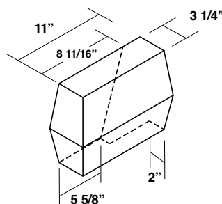
Gutter Corner Box for Standard Gutter 2:12 to 4:12 pitch or with Sculptured Eave (Right Hand Shown-Left Hand Opposite)
