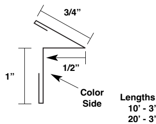
Alternate Rake Tie-In Trim
