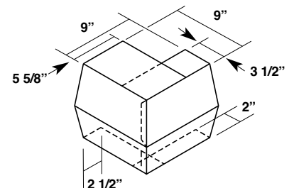
High Side Corner Box (Right Hand Shown-Left Hand Opposite) MLHCB
