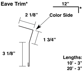
Sculptured Eave Trim* MLSCE
