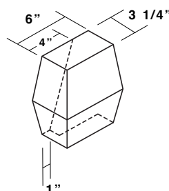
Gutter Corner Box for Sculptured Eave (Up to 4:12 Pitch) (Right Hand Shown-Left Hand Opposite)
