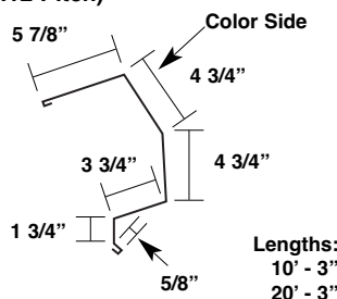
Fixed Ridge Flashing* (Up to 4:12 Pitch) MLFXR
