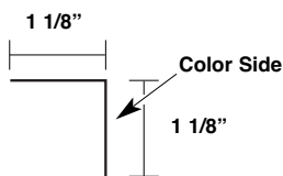
Insulation Angle Trim MLIA
