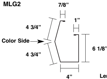
Gutter (Up to 2:12 Pitch) MLG2
