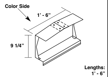
Fixed Peak Box (Up to 2:12 Pitch) MLFXPB2
