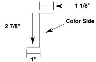
Zee Flashing ML3ZF
