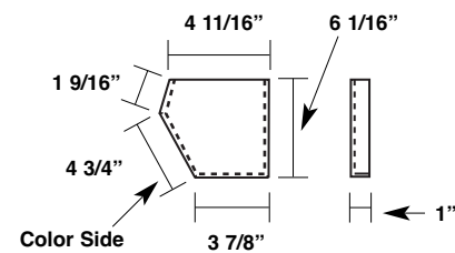
Gutter End Cap (Up to 2:12 Pitch) MLGE2
