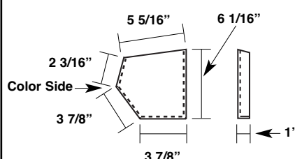
Gutter End Cap (2:12 to 4:12 Pitch) MLGE4
