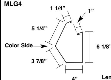
Gutter (2:12 to 4:12 Pitch) MLG4
