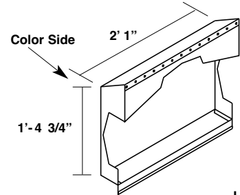
Floating Peak Box (2:12 to 4:12 Pitch) MLFLPB4
