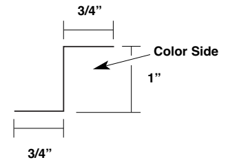
Gutter Strap ML-GS
