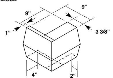
Outside Corner Box for Standard Gutter (Up to 2:12 Pitch) (Right Hand Shown - Left Hand Opposite) MLOCB
