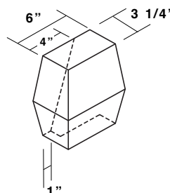
Gutter Corner Box for Sculptured Eave (Up to 4:12 Pitch) (Right Hand Shown-Left Hand Opposite)
