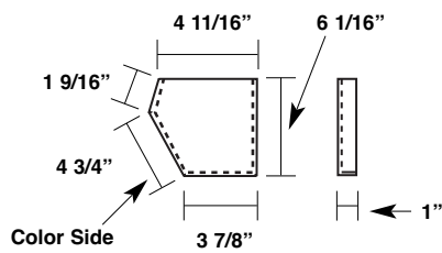
Gutter End Cap (Up to 2:12 Pitch) MLGE2
