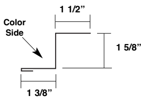
High Side Eave Trim* Up to 6:12 Pitch
