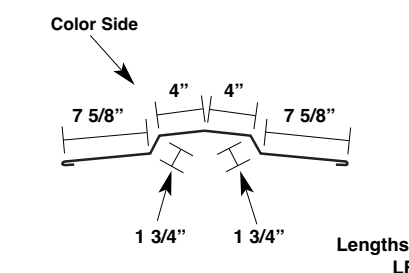
Floating Ridge Cap* Up to 6:12 Pitch
