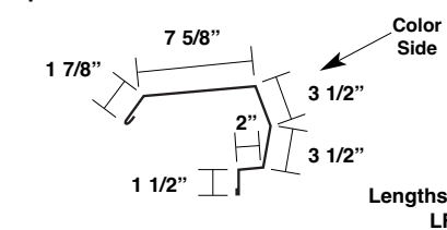
Floating Ridge Cap* Up to 6:12 Pitch
