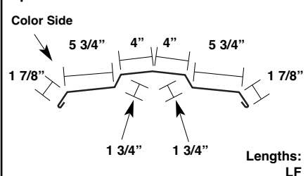
Alternate Floating Ridge Cap* Up to 6:12 Pitch
