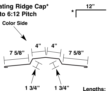
Alternate Floating Ridge Cap* Up to 6:12 Pitch
