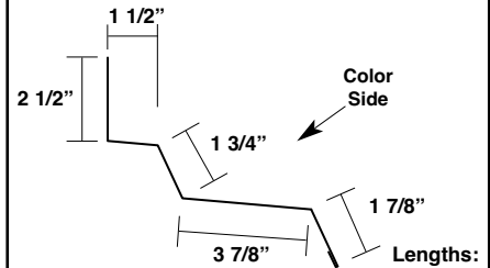
Fixed Ridge Cap* Up to 6:12 Pitch
