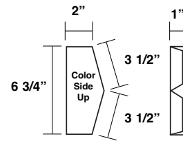
Rake Closure
