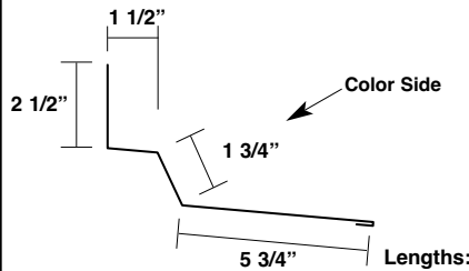
Alternate High Side Eave Trim* Up to 6:12 Pitch
