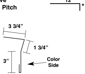
Sculptured Eave* Up to 6:12 Pitch
