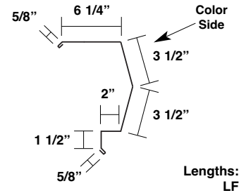
Rake Closure
