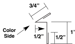
Rake Slide
