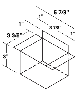
Lock-Seam Downspout Outlet - Standard
