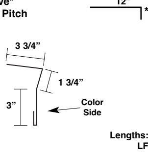
Sculptured Eave* Up to 6:12 Pitch
