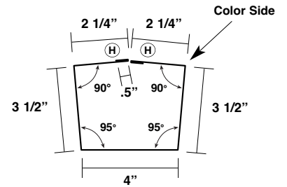
Lock-Seam Downspout
