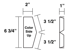
Rake Closure
