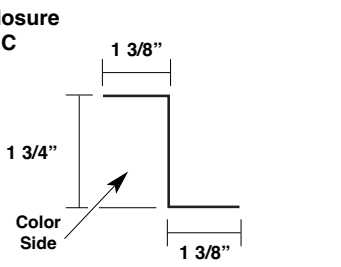
Vented Zee Closure
