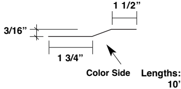
Zee Closure MDLZC
