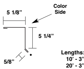
Vented Zee Closure
