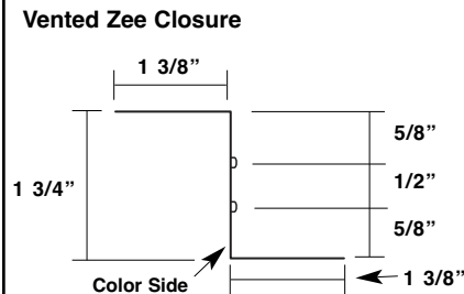
Vented Zee Closure
