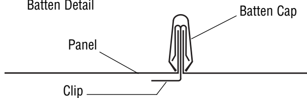
Medallion I Seam & Batten Detail
