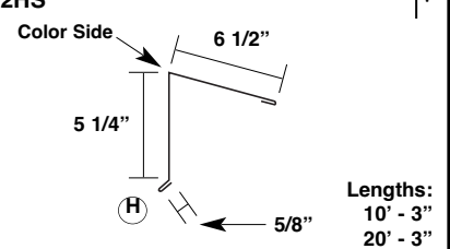
Ridge Flashing* MDRF
