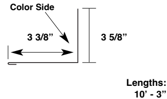
High Side Tie-In Trim* MDSW
