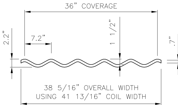
MET-TILE PROFILE
