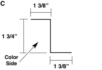
Zee Closure MDLZC
