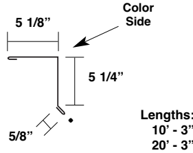
Vented Zee Closure
