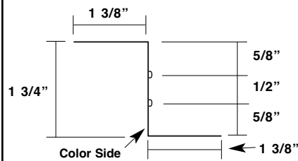
Vented Zee Closure
