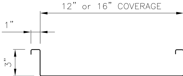
MCP PROFILE
