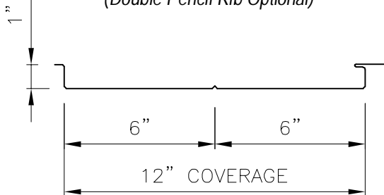
MARQUEE II PROFILE (Single Pencil Rib Optional)
