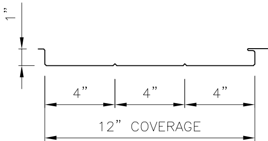
MARQUEE II PROFILE (Double Pencil Rib Optional)
