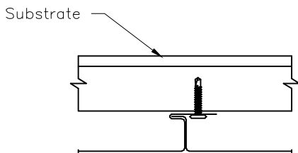
MARQUEE II SEAM
