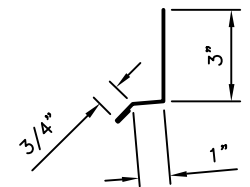
SIMPLE BASE TRIM
