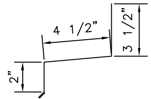
MASONRY WAINSCOAT TRIM
