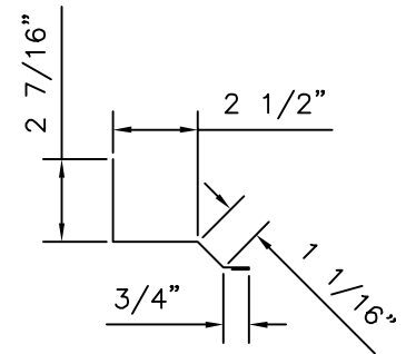
RAKE TIE-IN TRIM
