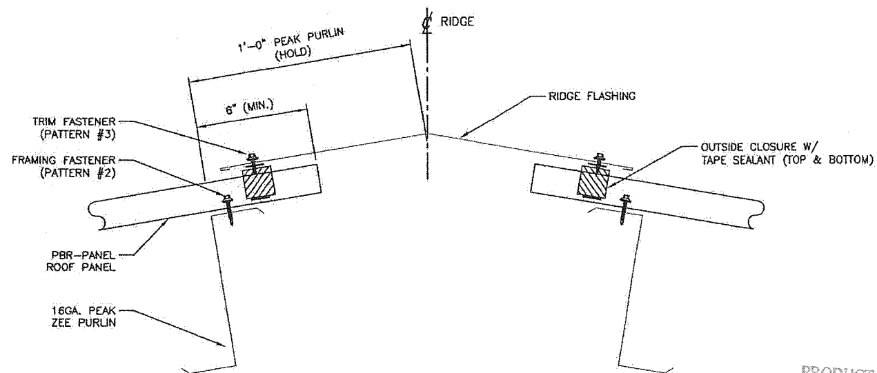
DETAIL @ RIDGE
