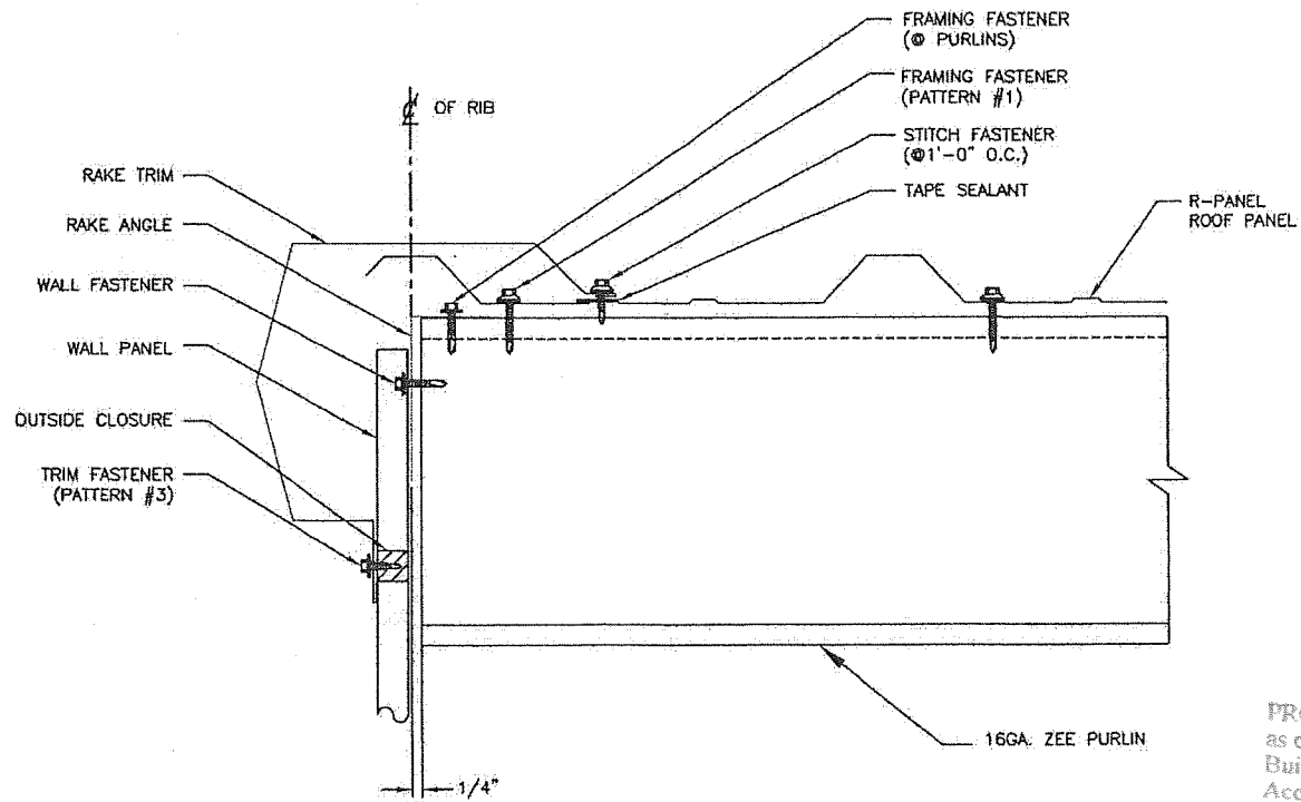
DETAIL @ RAKE
