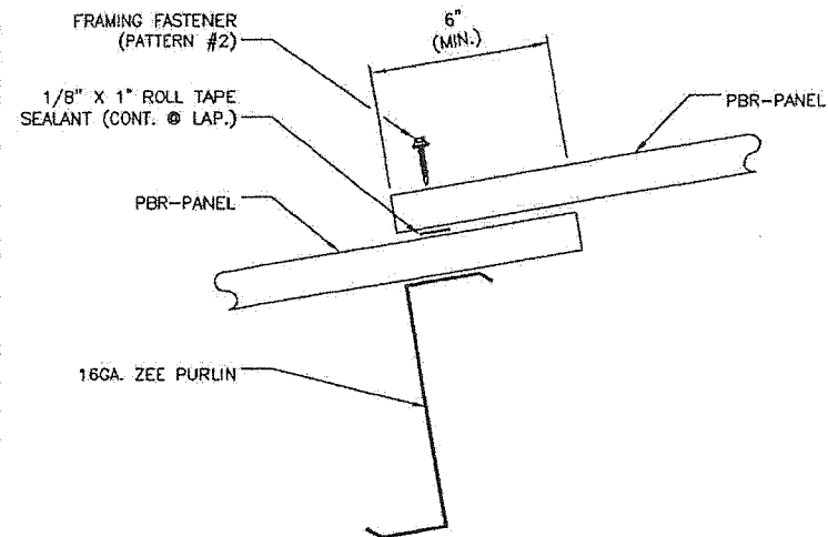
DETAIL @ PANEL LAP
