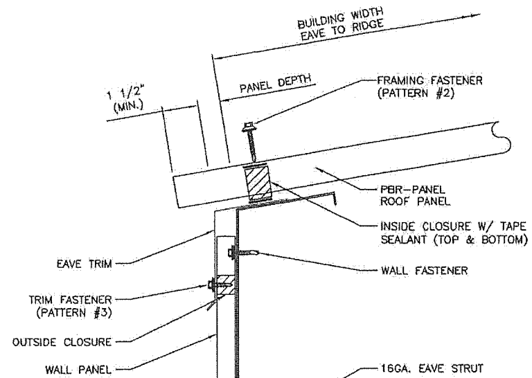
DETAIL @ EAVE
