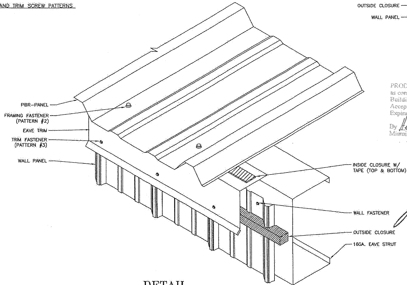
DETAIL @ EAVE (ISOMETRIC VIEW)
