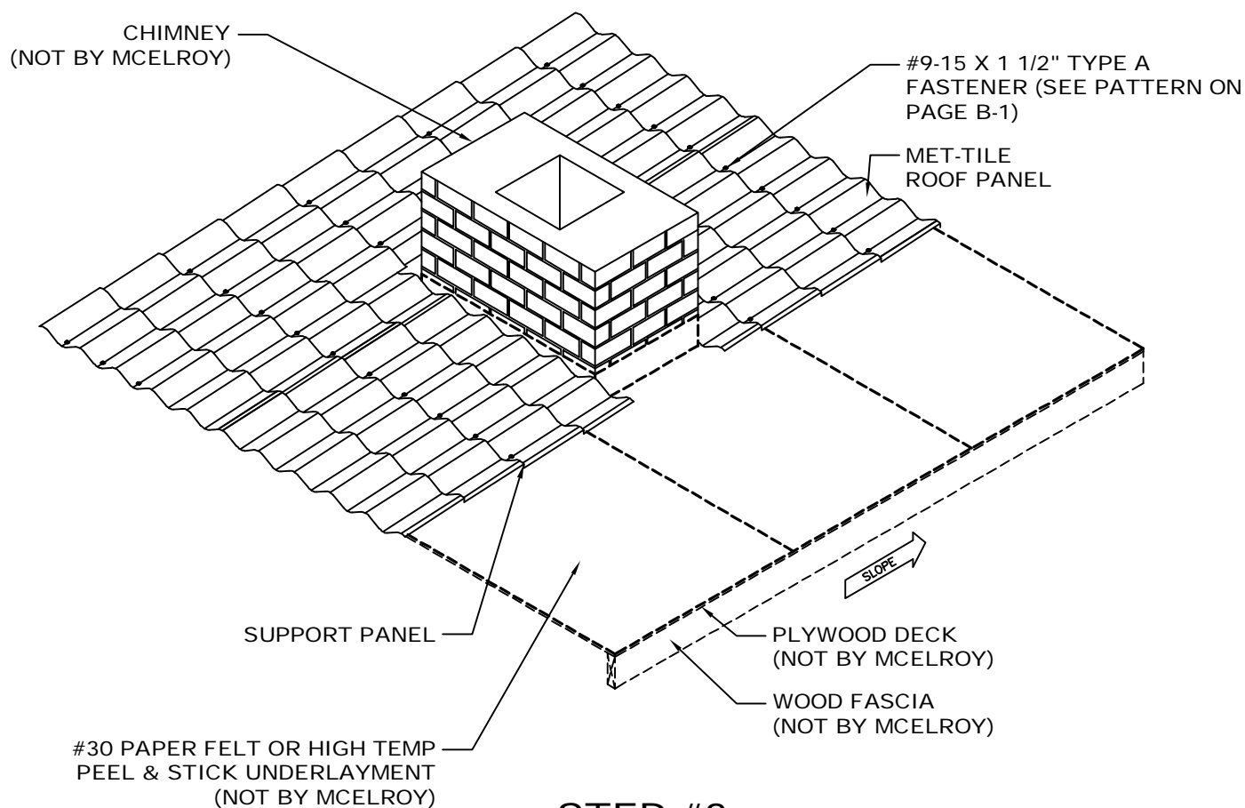
STEP #3
