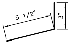
COMMERCIAL HI-SIDE TIE-IN TRIM
