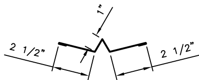
VALLEY COVER TRIM
