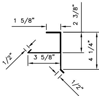
COMMERCIAL RAKE TRIM
