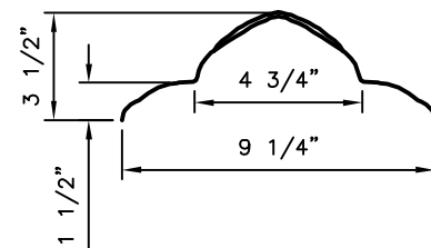
CONTOURED HIP TRIM
