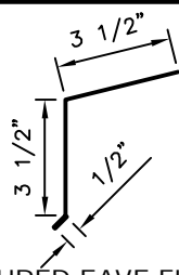
CONTOURED EAVE FLASHING
