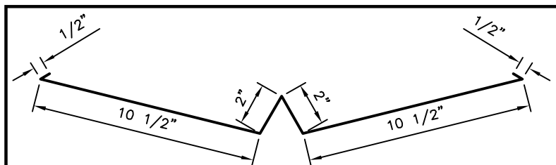
VALLEY TRIM
