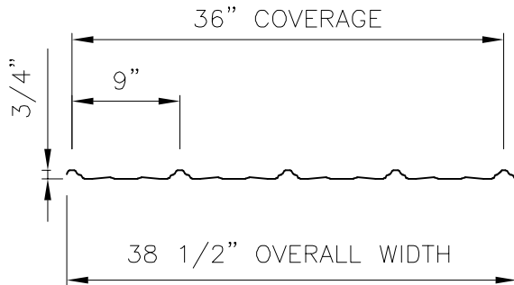
MESA PANEL PROFILE
