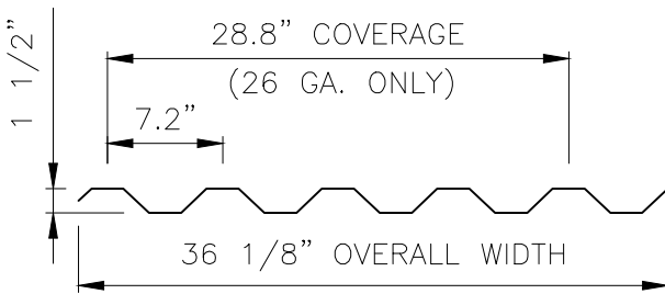
MEGA-RIB PROFILE (NARROW PANEL)
