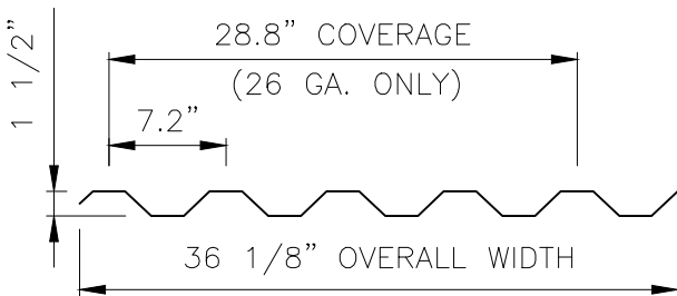
MEGA-RIB PROFILE (NARROW PANEL)
