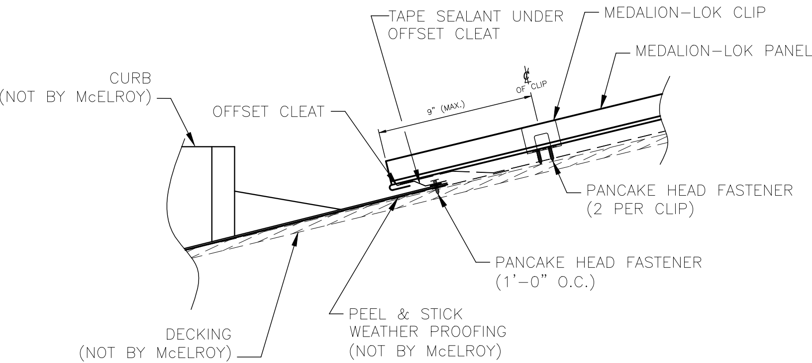
DETAIL "E"
