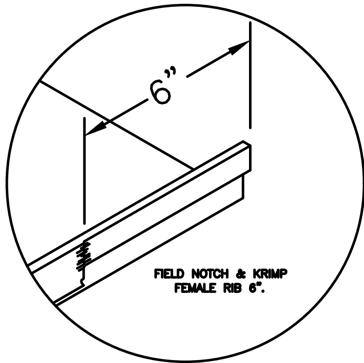
DETAIL "B"
