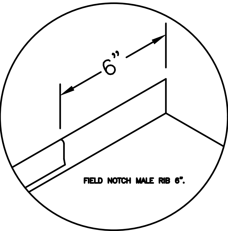
DETAIL "A"
