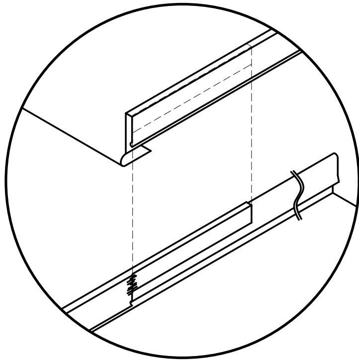
DETAIL "D"
