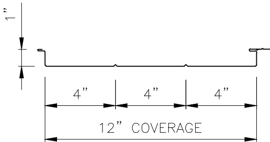
MARQUEE-LOK PROFILE (Double Pencil Rib Optional)
