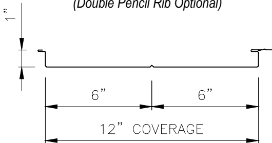
MARQUEE-LOK PROFILE (Single Pencil Rib Optional)
