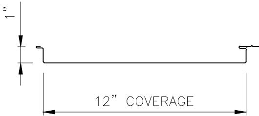
MARQUEE-LOK PROFILE (Flat Pan Standard)
