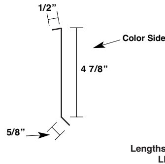
Floating Headwall Trim MT-192
