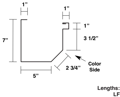
Floating Ridge Trim MT-189
