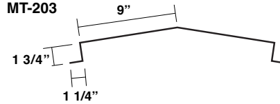
1 3/4" Offset Hip/Ridge Plate MT-203
