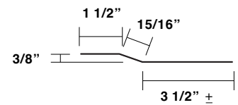
Low Eave Plate MT-185
