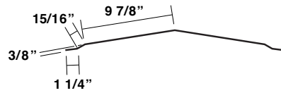
3/8" Offset Hip/Ridge Plate MT-202
