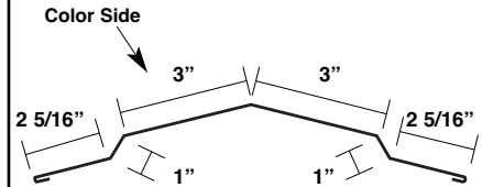
Ridge Cap* MODRC13
