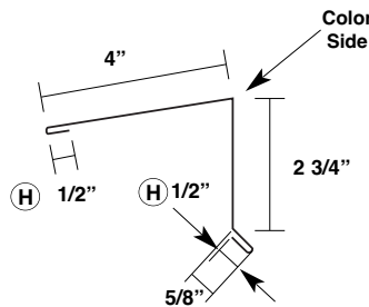
M 2.75" Peak Trim MODM275P
