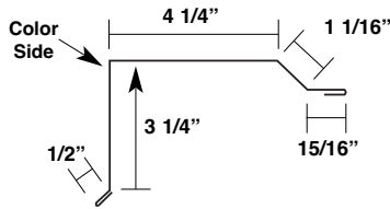
Denver Rake Trim MODDR
