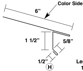
M 1.5" Eave Drip MODM15ED
