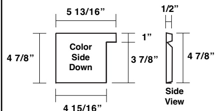
Gutter End Cap for Standard Box Gutter & Flanged Box Gutter MT-68R = Right End Cap MT-68L = Left End Cap
