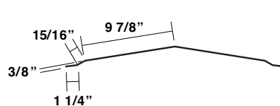
3/8" Offset Hip/Ridge Plate MT-202
