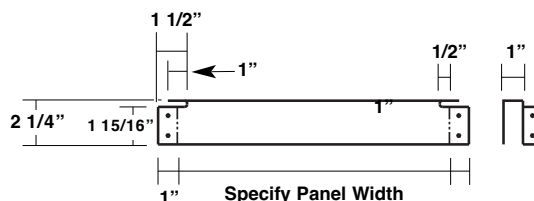
238T Metal Closure @ Ridge MT-238T-CLOS
