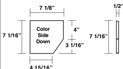
Gutter End Cap for 7" Box Gutter MT-69R = Right End Cap MT-69L = Left End Cap
