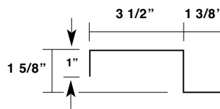
238T Retrofit Clip Eave Plate MT-188
