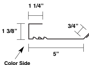
Perforated "J" Channel (Use with MT-3 Vented Ridge Cap and MT-154 Vented Headwall) MT-133
