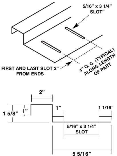
High Floating Eave Plate MT-208
