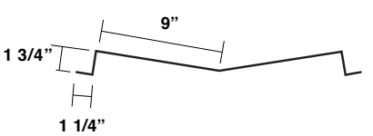
1 3/4" Offset Valley Plate MT-201
