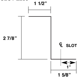
Slotted Starter Zee MT-SLOT-Z238
