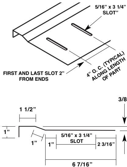
Low Floating Eave Plate MT-209
