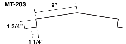
1 3/4" Offset Hip/Ridge Plate MT-203
