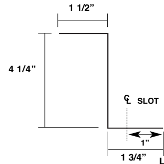
238T Slotted Rake ZEE - Retrofit MT-SLOT-Z238-RETRO
