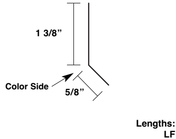
Flanged Box Gutter MT-62
