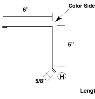
Alternate Rake Trim MT-183
