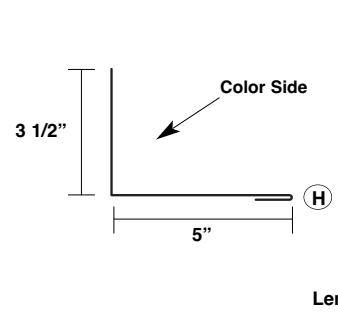
Standard Sidewall Trim MT-34
