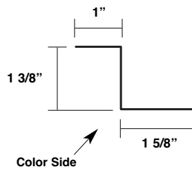
138T Notched Zee Closure MT-14N
