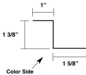
138T Zee Closure MT-14
