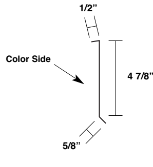
Rake Support Cleat MT-156
