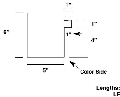
Gutter End Cap for Standard Box Gutter & Flanged Box Gutter MT-68
