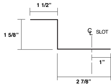
138T 16 GA. Galv Slotted Starter Zee MT-SLOT-Z138T ITEM #: 21633
