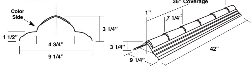
Contoured Ridge / Hip Trim
