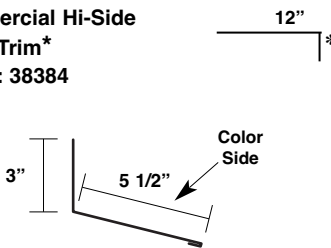
Commercial Hi-Side Tie-In Trim*
