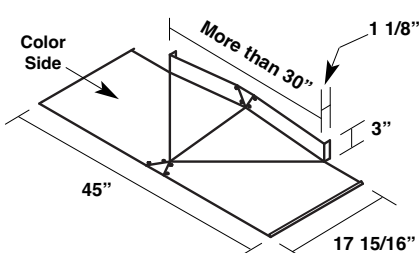
Cricket (Finished) Item #: 38417
