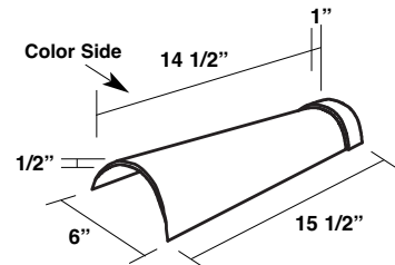
Commercial Ridge / Hip Trim* Item #: 38419
