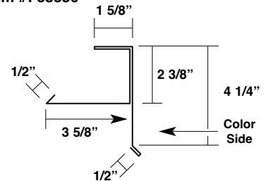
Commercial Rake Trim
