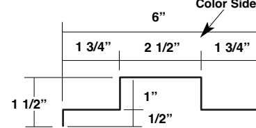
Counter Flashing Trim
