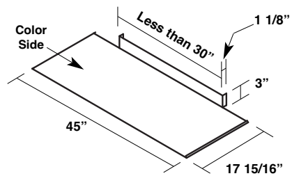
Saddle (Finished) Item #: 38418
