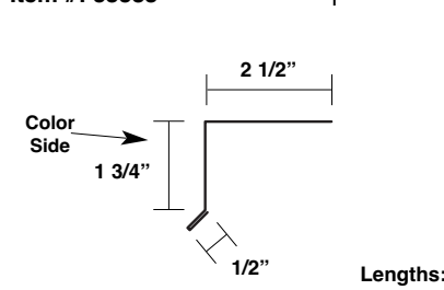
Contoured Hi-Side Tie-In Trim
