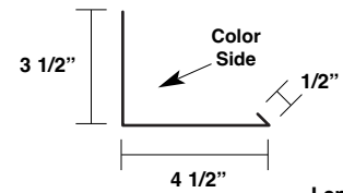
Commercial Rake Trim
