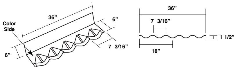
Contoured Hi-Side Tie-In Trim
