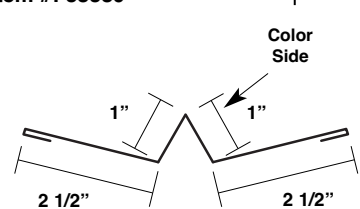
Valley Cover Trim*
