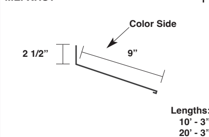
Floating Ridge Flashing* (Up to 4:12) MFLR4
