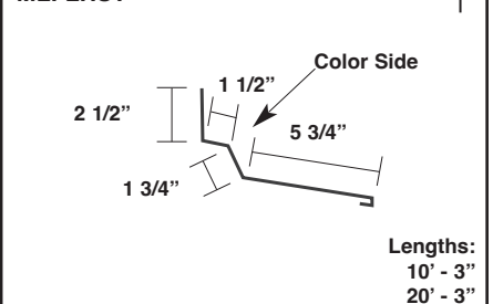
Fixed Peak Box (Up to 2:12 Pitch) MLFXPB1
