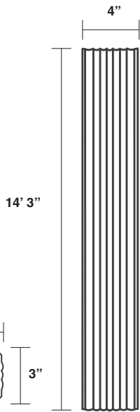
Lock-Seam Downspout - Corner (Right Hand Corner Shown)
