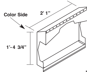
Floating Peak Box (Over 2:12 to 4:12 Pitch) MLFLPB4
