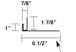
Overhead Door Flashing 6 1/2" (P-JF-B-6 1/2)
