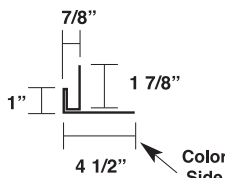
Overhead Door Flashing 4 1/2" (P-JF-B-4 1/2)
