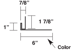
Overhead Door Flashing 6" (P-JF-B-6)
