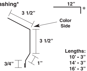
Shingle Rake Trim (P-SRT)
