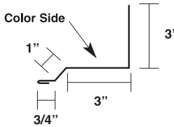
Rake Tie-In Trim (P-EWF)
