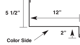
Eave Flashing* (P-EF)*
