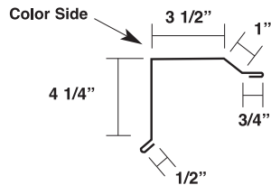
Hi-Side Tie-In* (R-SW)
