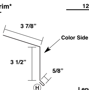
Eave Drip 1.5" MRAM15EDT
