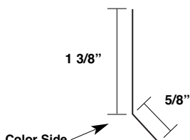
Perimeter Cleat MRAPC
