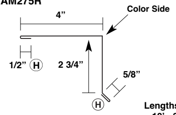
Rake Trim 2.75" MRAM275R
