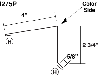
2.75" Peak Trim MRAM275P
