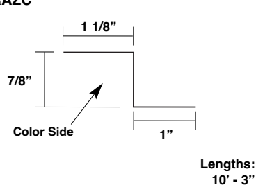
High Side Tie-In Trim* MRESW
