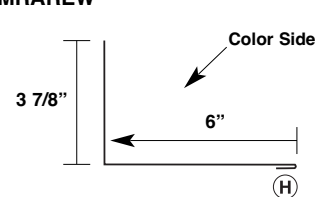
Sidewall Trim MRAREW
