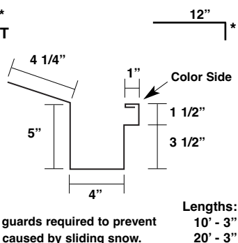
Gutter Strap MRD-GS
