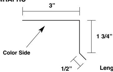
Fixed Rake Cleet MRAFC
