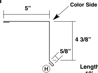
Rake Tie-In Trim MRAEW
