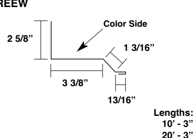
Vented Zee Closure MRAVZC
