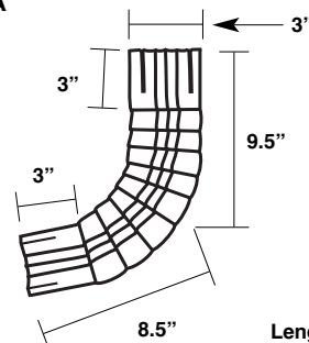
"A" Style Downspout Elbow BBPELA
