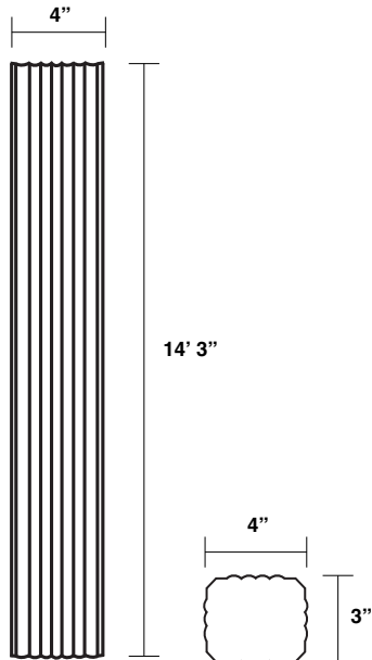
Downspout BBPDS
