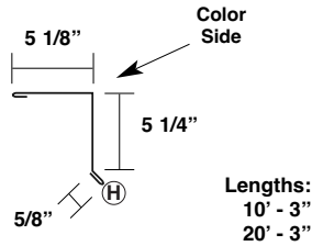
Vented Zee Closure
