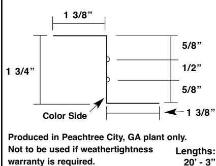
Hip Flashing* MDHF
