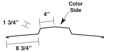
Floating Ridge Flashing* Up to 4:12 Pitch MFLR1
