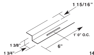
High Floating Rake Plate Item #: 17482
