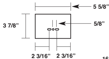
Bearing Plate Item #: 94599 Primed Item #: 203541 Galvanized
