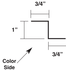
Gutter End Cap Over 2:12 TO 4:12 Pitch MX2GEC4
