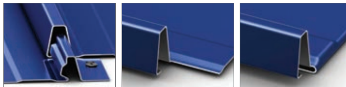
Factory Eave Notch
