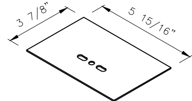
BEARING PLATE
