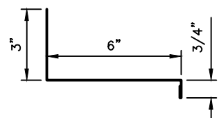
RAKE TIE-IN TRIM (ALT.)
