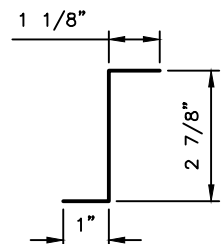
ZEE CLOSURE
