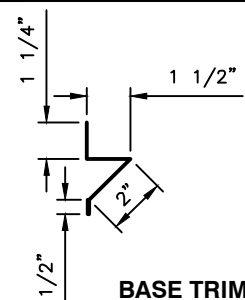
BASE TRIM
