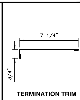
RAKE SLIDE
