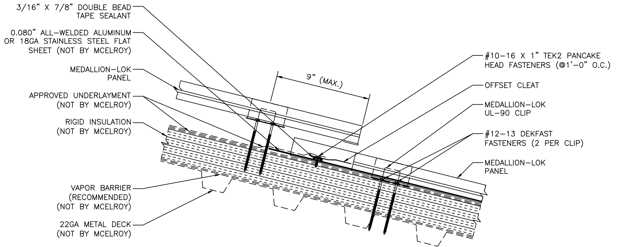
DETAIL "E"
