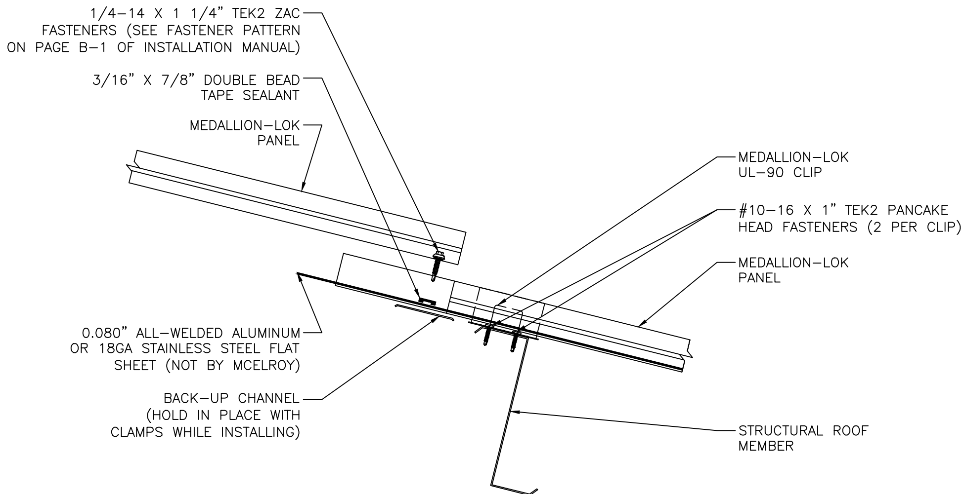
DETAIL "E"
