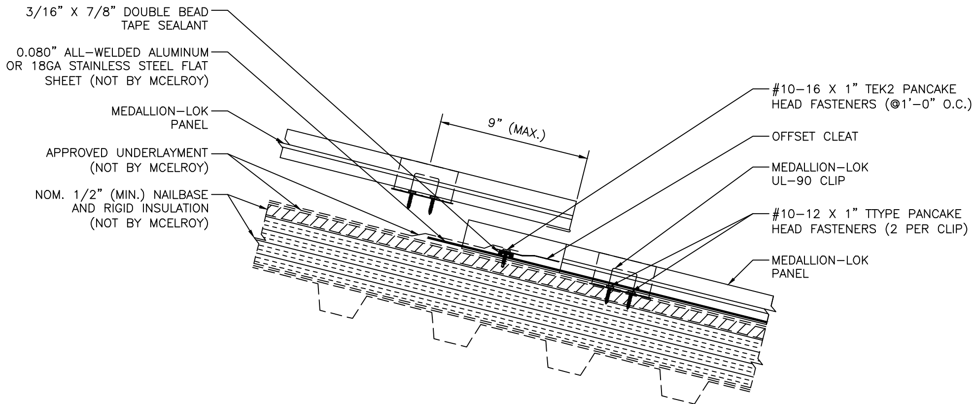
DETAIL "E"
