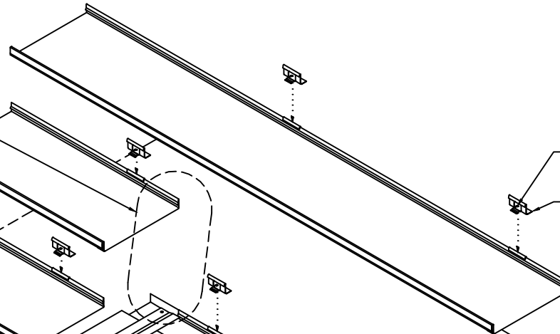
DETAIL "C"
